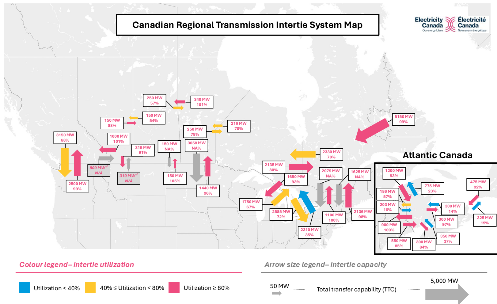
Figure 2 – Current state of Canadian interprovincial intertie system. Arrow sizes represent the TTC; arrow colours represent the intertie utilization. 3,4 N/A data and grey arrows indicate where data was not available.
